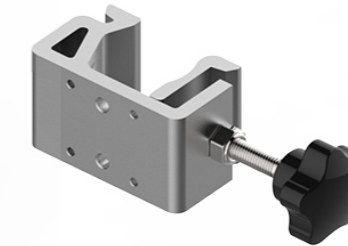
Model:CL001-00 Functional clamps 30*30mm Model:CL001-008-02 Functional clamps 25*25mm Model:CL001-11-01 Functional clamps 19*19/20*20mm
